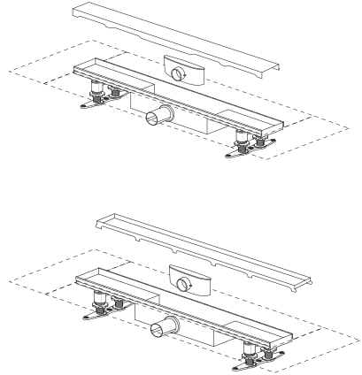
RainDrain Compact 56162800 - 56185000
